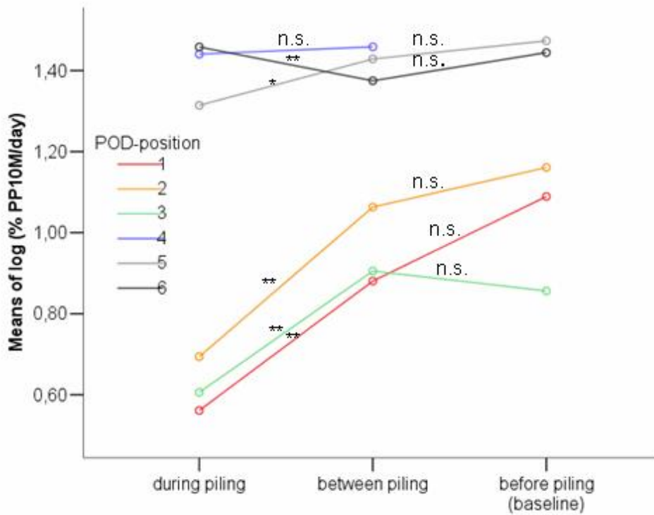
Fig. 14 a: Means of log-transformed % of PP10M/day for all POD-positions on days before, between and during pile driving events as predicted by the model.
