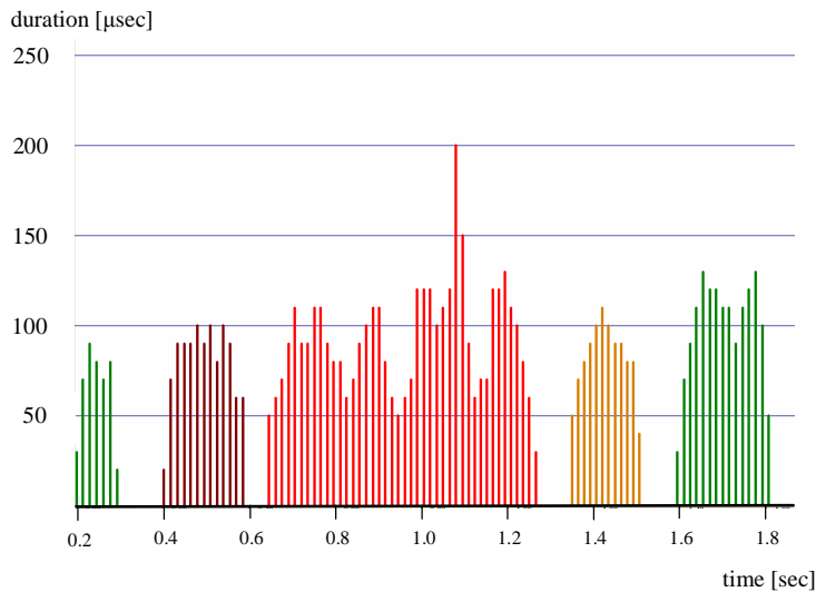
Fig. 4: Example of a registered porpoise click sequence divided by different click trains, shown as series of vertical bars (clicks), where the time [sec] is shown on the x-axis and duration of a click on the y-axis.
