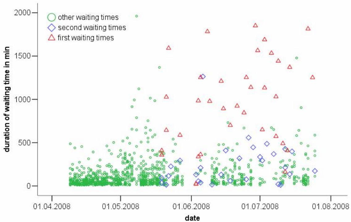
Fig. 17 c: Duration of waiting time between porpoise encounters in min by date of occurrence for POD-position 3.
