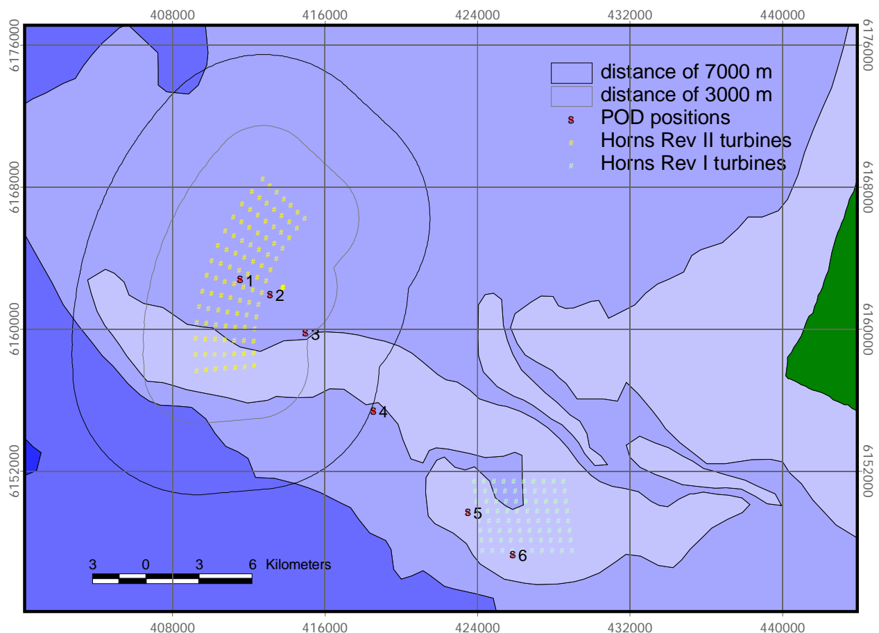
Fig. 6: Study area and position of wind farms and PODs.
