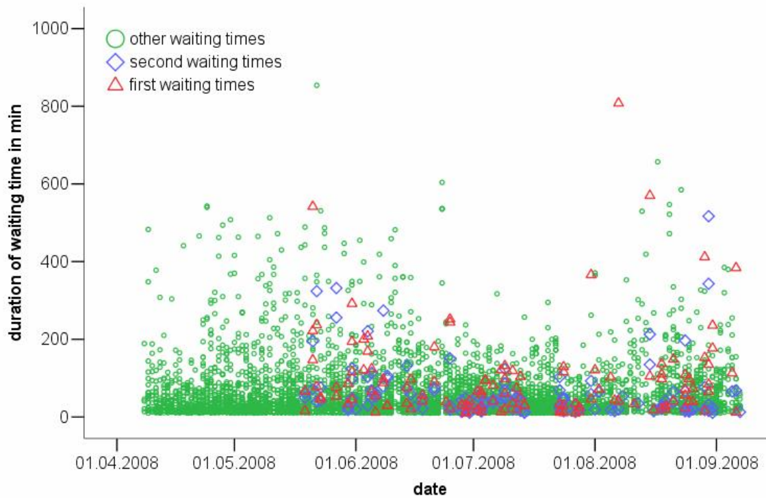
Fig. 17 f: Duration of waiting time between porpoise encounters in min by date of occurrence for POD-position 6.
