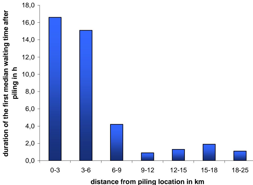
Fig. 19 a: Duration of the median first waiting times after piling by distance in km from the piling location.
