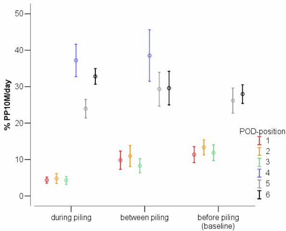
Fig. 14 b: Means and 95 % confidence intervals of % of PP10M/day for all POD-positions on days before, between and during pile driving events.
