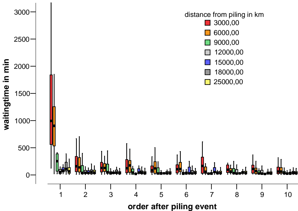
Fig. 18: Boxplots showing medians and 95 % confidence intervals of duration of waiting time in min between porpoise encounters by their order after the last piling event and the different distance categories.
