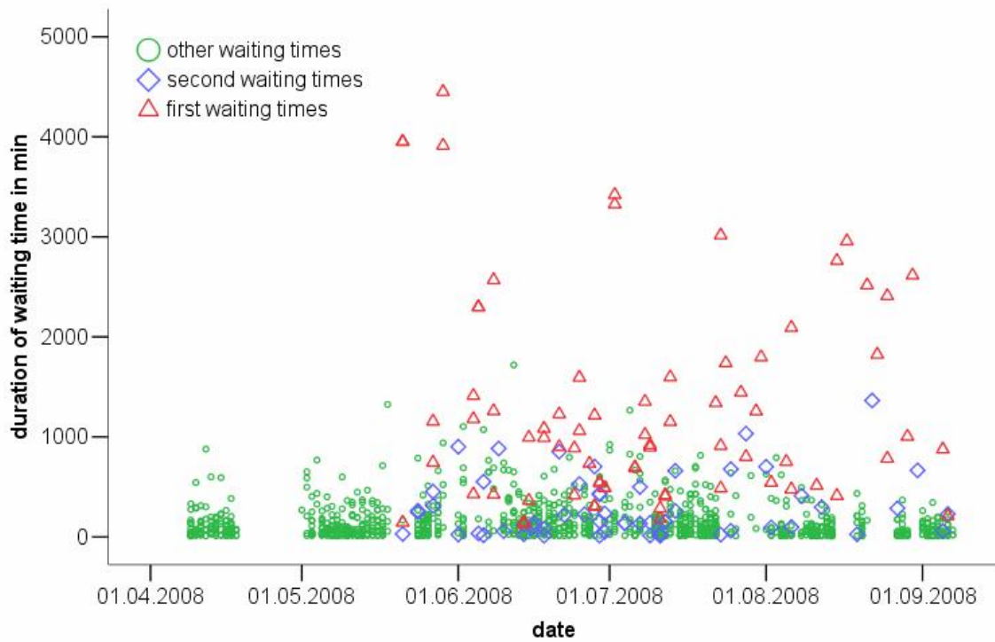
Fig. 16 a: Duration of waiting time between porpoise encounters in min by date of occurrence for POD-position 1.
