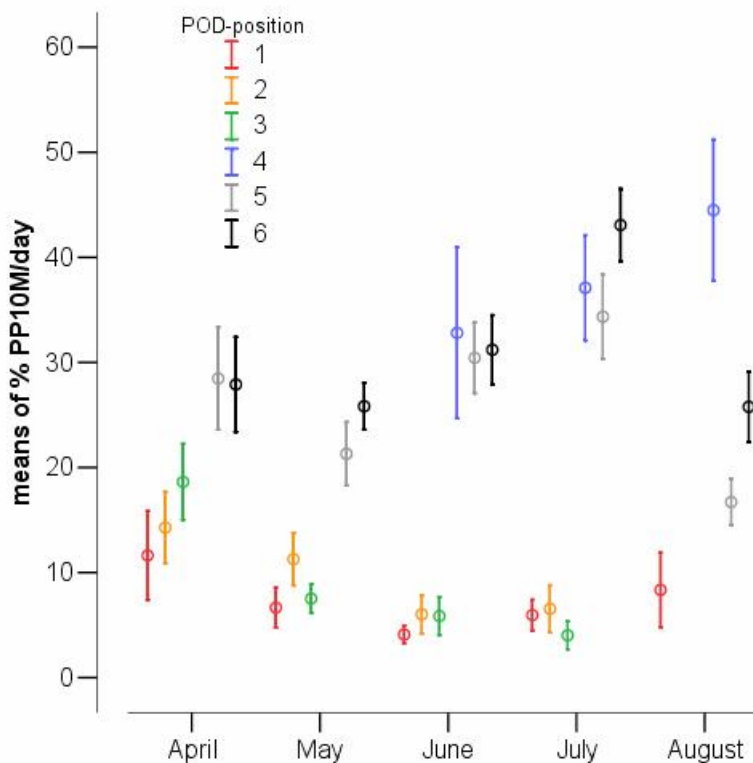
Fig. 12: Seasonal change in PP10M/dy at the different POD-positions around Horns Rev II.
