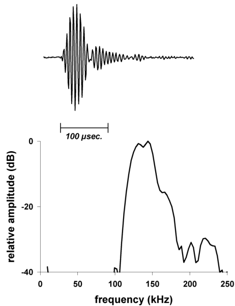
Fig. 1: Waveform (above) and frequency spectrum of a porpoise echo-location click (from Verfuß et al. 2004).
