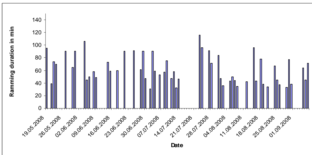
Fig. 10: Timing of piling events depicted as number of minutes that pile driving took place on the day where an event was finished.
