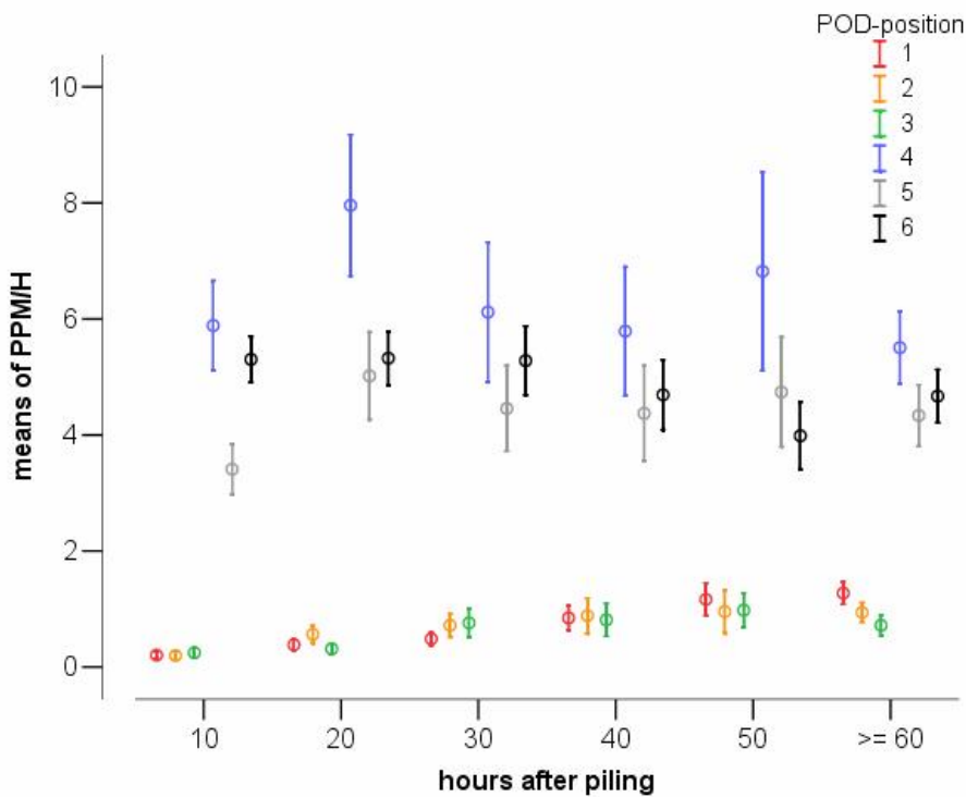
Fig. 15 b: Raw means and 95 % confidence intervals of PPM/Hour for the different POD-positions with time after the piling event in 10 hour steps.
