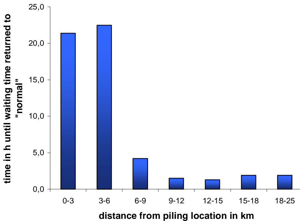
Fig. 20 b: Time in hours that it takes for median waiting times to return to “normally expected” values by distance in km from the piling location.
