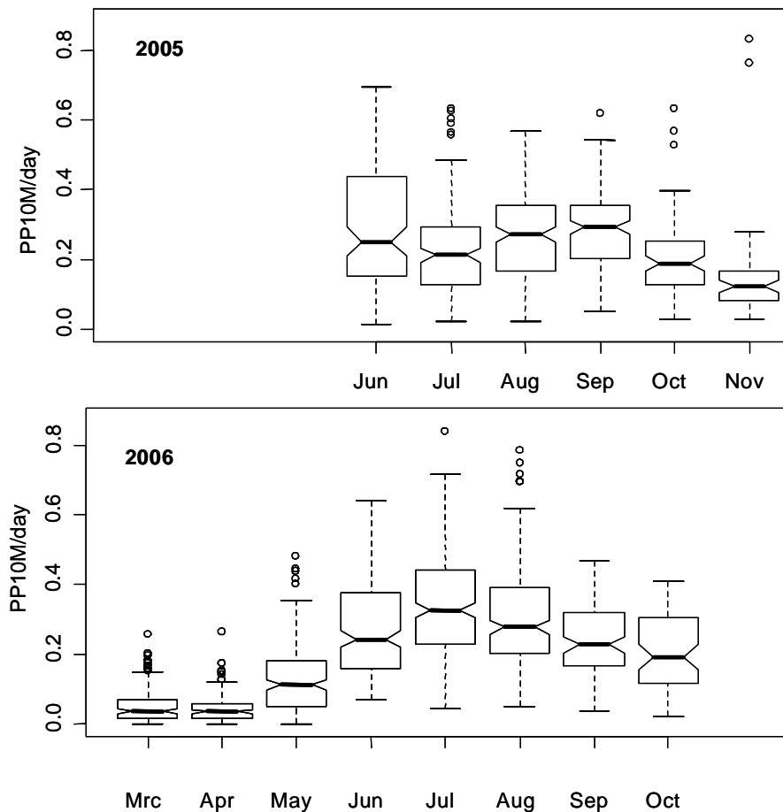
Fig. 12b: Seasonal change in PP10M/day during 2005 and 2006 in the area around Horns Rev I.
