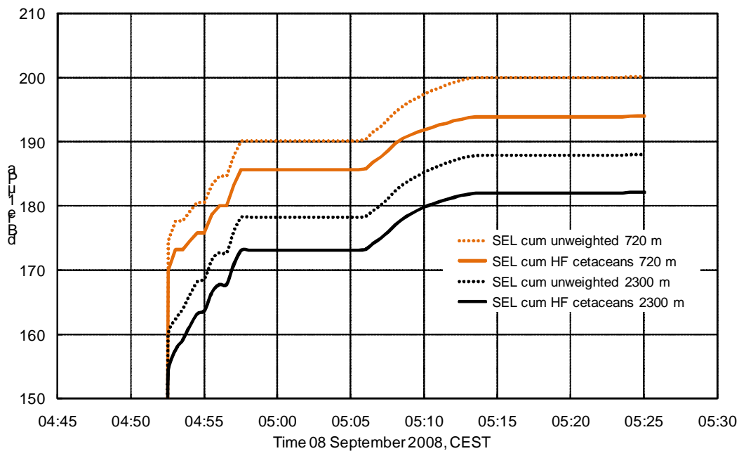
Fig. 21: Cumulative SELs for two measurement distances during pile driving (from Betke 2008).
