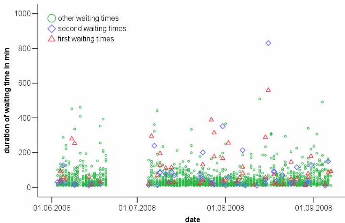
Fig. 17 d: Duration of waiting time between porpoise encounters in min by date of occurrence for POD-position 4.
