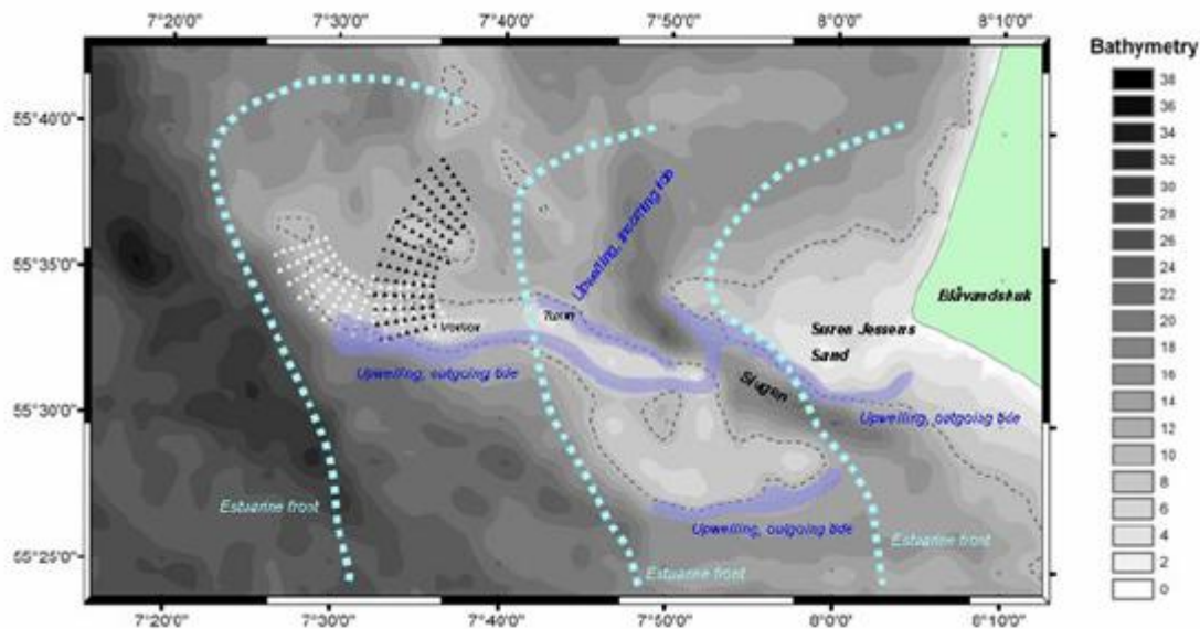
Fig. 22: Map showing the physical environment of Horns Rev. The 10 m (dotted line) depth contour, typical up-welling zones (blue raster) and potential position of the estuarine front (light blue dotted line) are indicated. Taken from Skow et al. (2008).
