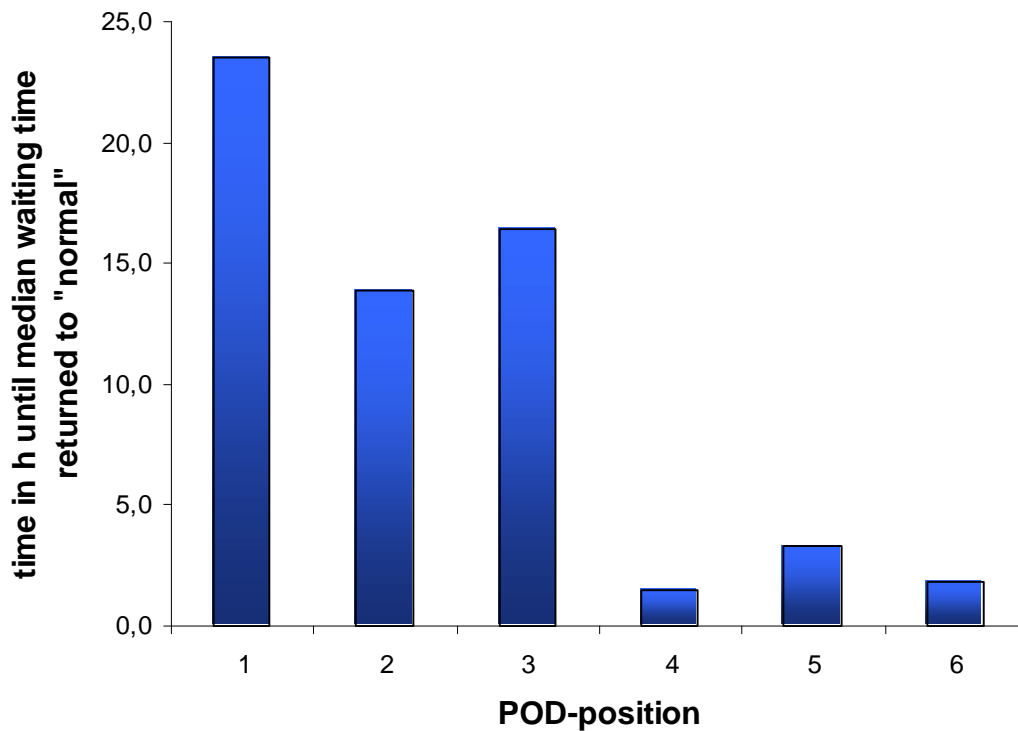
Fig. 18 b: Time in hours that it takes for median waiting times to return to “normally expected” values at the different POD-positions.
