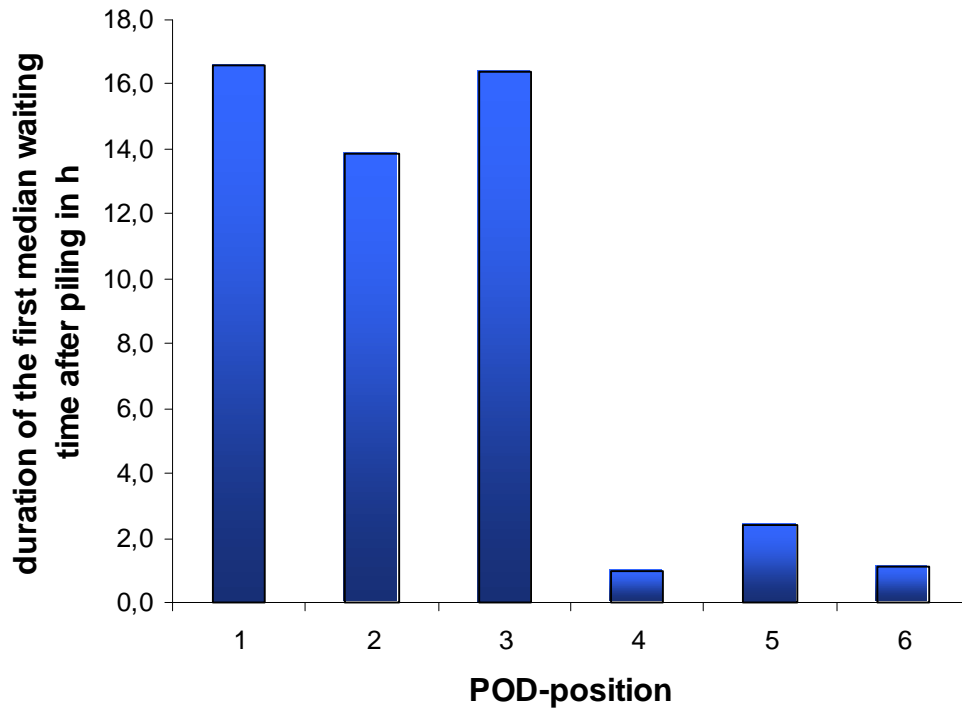
Fig. 17 a: Duration of the first median waiting time after piling for the different POD-positions.
