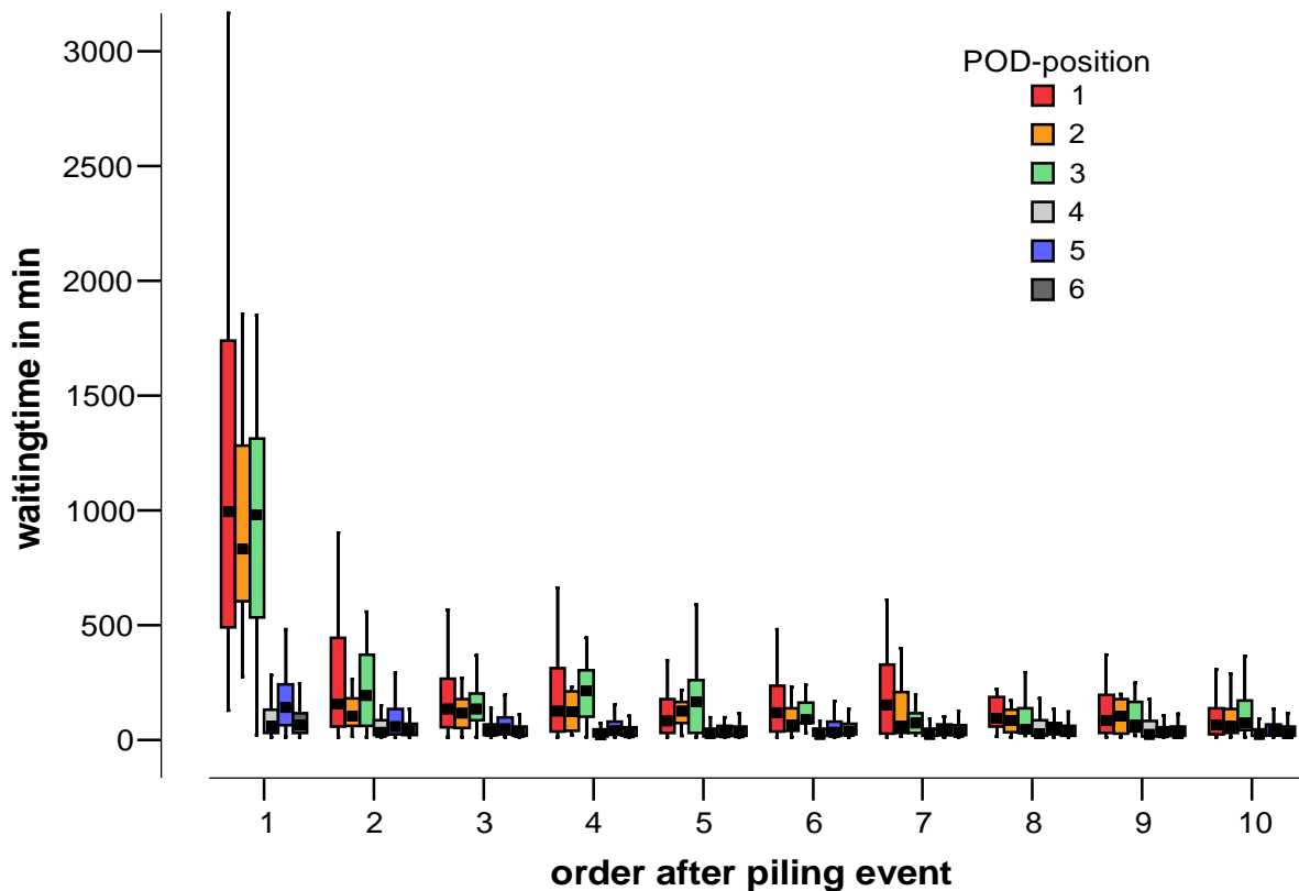
Fig.16. Boxplots showing medians and 95 % confidence intervals for duration waiting time in min between porpoise encounters by their order after the last piling event and the different POD-positions.
