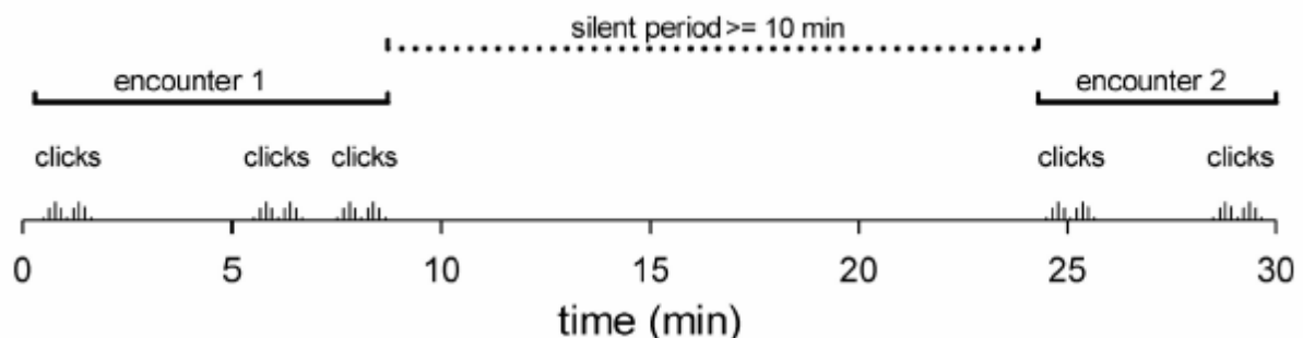
Fig. 11: Definition of “encounter” and “silent periods (= waiting time)” (from Benke et al. 2003).
