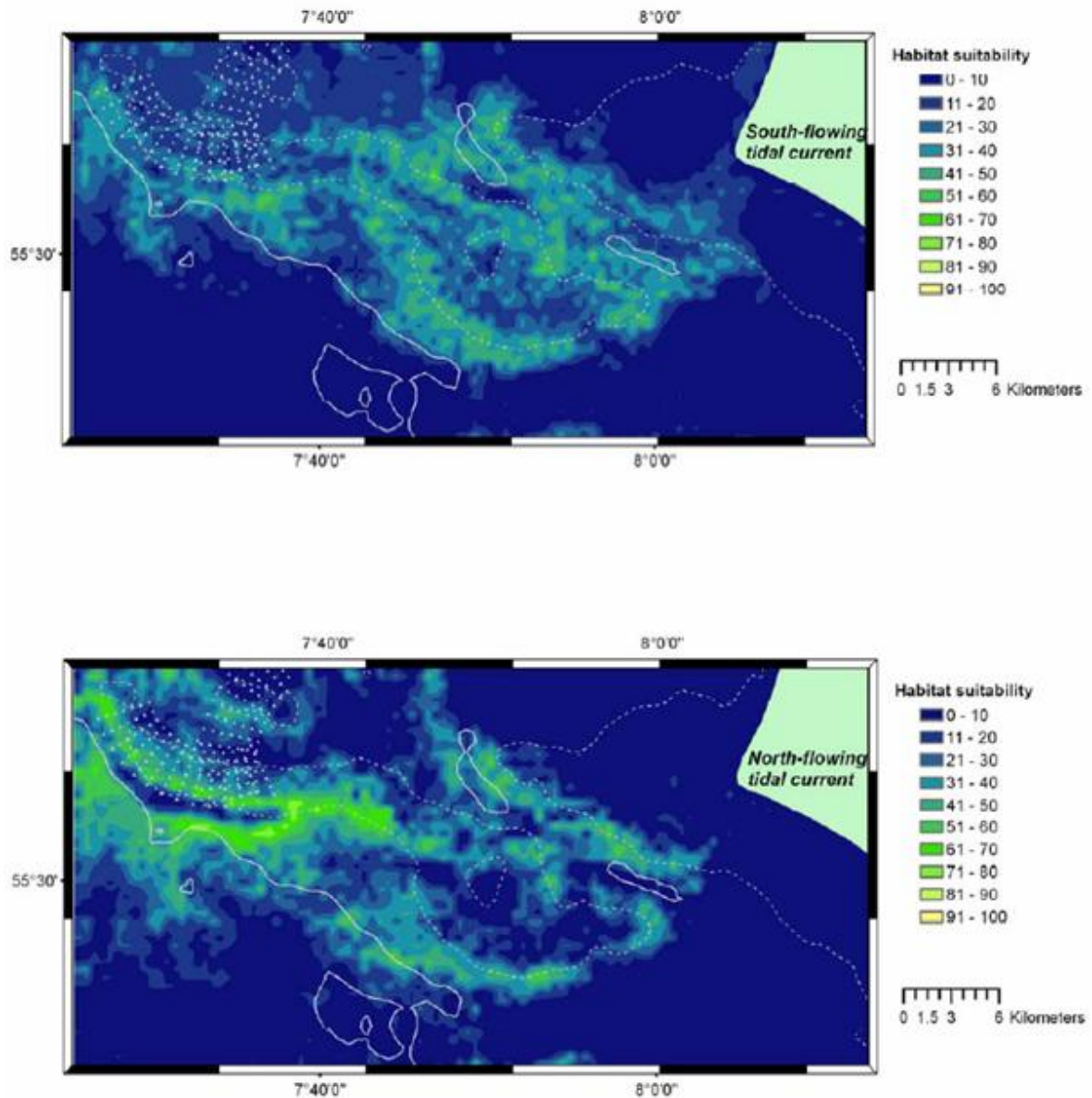
Fig. 23: Habitat suitability of harbour porpoise modelled from ship-based sightings during periods of south-flowing (above) and north-flowing (below) tidal currents (selected surveys). Taken from Skov et al. (2008).
