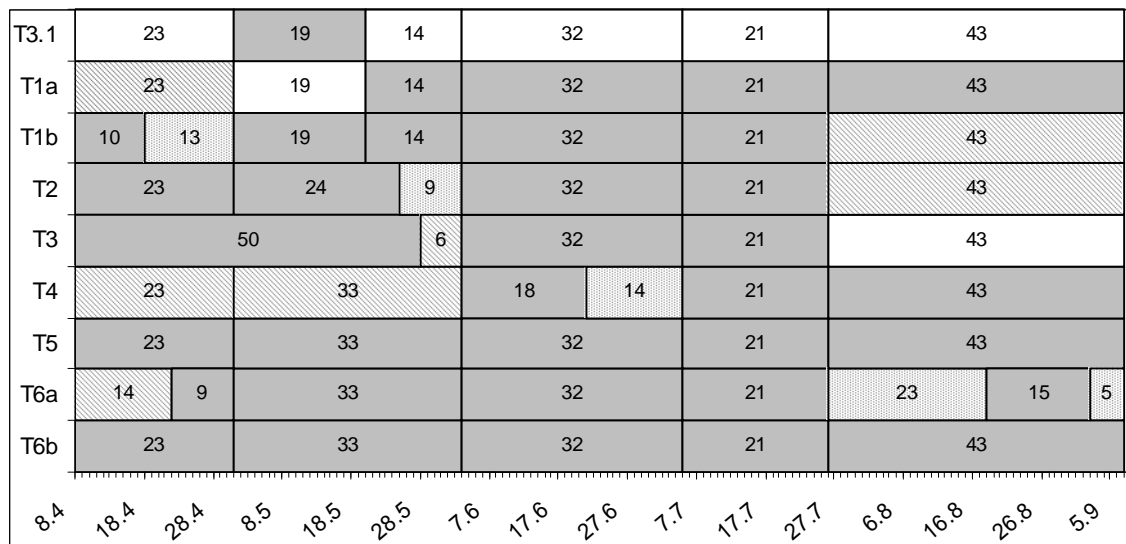
Fig. 9: Recorded data of PODs placed at different positions in relation to the offshore wind farm Horns Rev II. Vertical black lines show changes of PODs. Grey bars: POD recorded data, hatched bars: POD deployed but lost, dotted bars: POD deployed but did not record data; white bars: no POD deployed.
