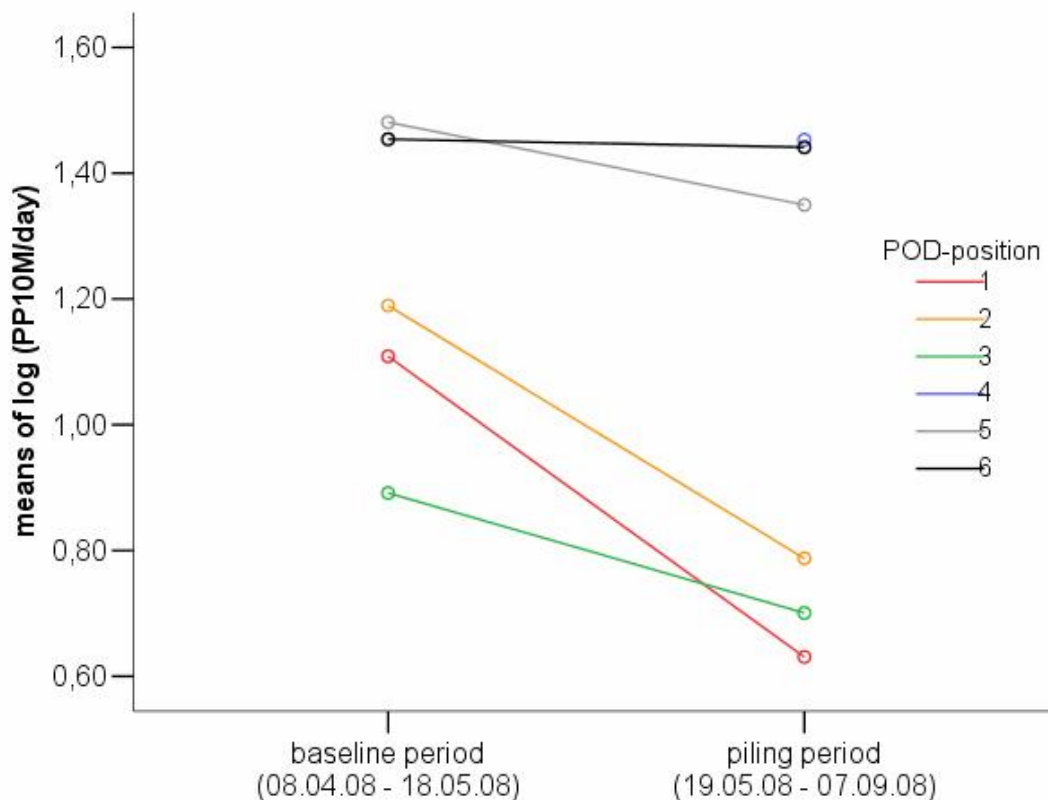
Fig. 13: Means of log-transformed porpoise positive ten minutes / day during the baseline and pile driving period as predicted by the model.
