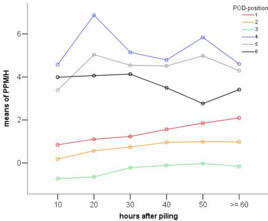
Fig. 15 a: Estimated marginal mean of PPM/Hour for the different POD-positions with time after the piling event in 10 hour steps as predicted by the model.
