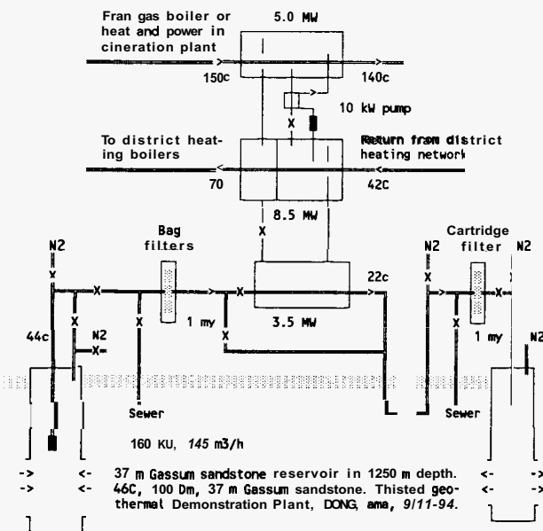
Fig. 1 : Thisted Geothermal Plant
