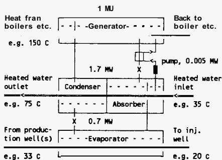
Fig.3: Absorption heat pump concept
